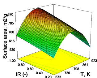
Figure 3. Three-dimensional plot of surface area of DPAC
