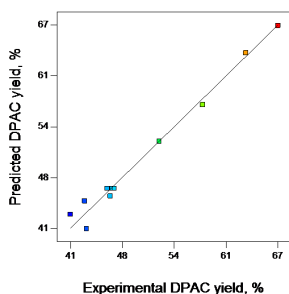
Figure 1.a. Predict versus experimental yield of DPAC
