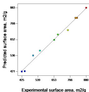
Figure 1.b. Predict versus experimental surface area of DPAC
