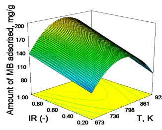
Figure 4. Three-dimensional plot of MB adsorbed
